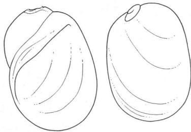
FIGURE 10.—Shells of Lymnaea newcombi from Hanakapiai Stream, Kauai (BBM 15571), shell-height 5 mm. The right specimen from above.
