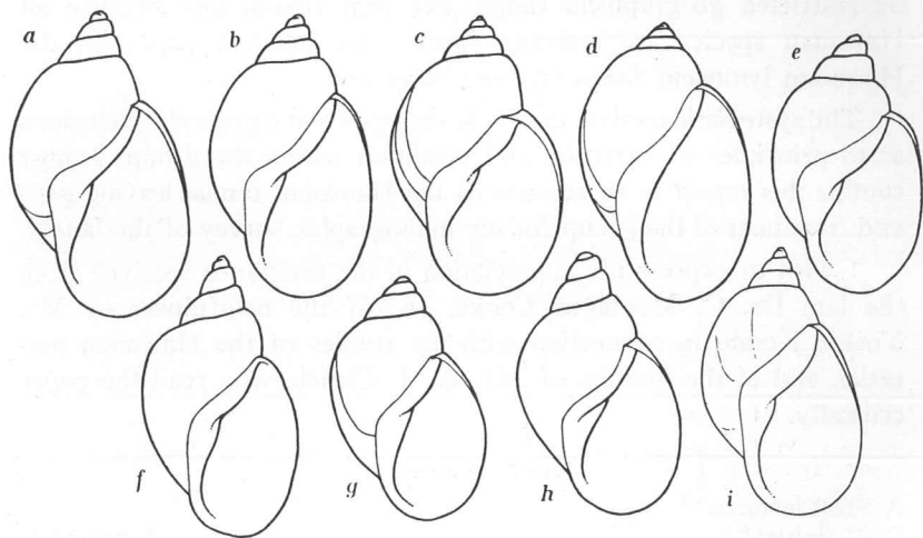
FIGURE 1.—Shells of Lymnaea volutata : a, b , from Kalalau Valley, Kauai (BBM 15633 and BBM 15645), shell heights 10 and 8.5 mm.; c , from Kailua, Oahu (BBM 168179), height 12 mm.; d , from Kewalo, Oahu (BBM 14765), 12 mm.; e, f , from Manoa, Oahu (BBM 14768), heights 8 and 9 mm.; g, h , from Nuuanu, Oahu (BBM 14764), heights 7 and 7.5 mm.; i , from Kalalau Valley, Kauai (BBM 15633), height 9 mm.
